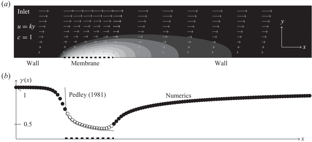
FIGURE 7. Comparison between our numerical method and Pedley’s analytical solution for a shear flow above a membrane as shown in (a). To the left, a solution of concentration c=1 is entering the computational domain with a velocity profile (u, v) = (ky, 0) . As the solution passes above the membrane, the flow and concentration profiles are perturbed, creating a characteristic boundary layer. Also shown in (a) are concentration contours (scale bar in figure 3c) and velocity arrow plot for k=25 and Pe=10 . (b) Plot of the numerically computed concentration at the lower wall \gamma(x) as a function of position x (open circles at the membrane, and solid circles on the wall). The solid line represents Pedley’s analytical solution (Pedley 1981).
